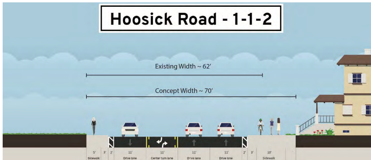
FIGURE 3.1 – WIDENING CONCEPT (1-1-2)
